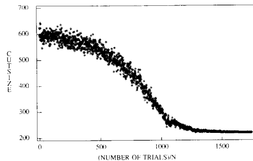
Figure 13. The evolution of the solution value during annealing on G_{500} . (Time increases, and hence, temperature decreases along the X -axis. The Y -axis measures the current solution value, that is, the number of edges in the cut plus the imbalance penalty.)
