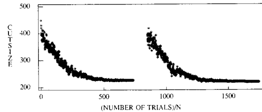
Figure 15. Comparison of the tail of an annealing run where INITPROB = 0.4 and MINPERCENT = 2% with an entire annealing run where INITPROB = 0.9 and MINPERCENT = 1%.
