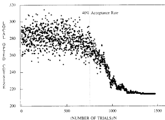
Figure 14. The evolution of Local-Opt( S ) during annealing on G_{500} , where S is the current solution and Local-Opt( S ) is the cutsize obtained by applying Local Opt to S .
