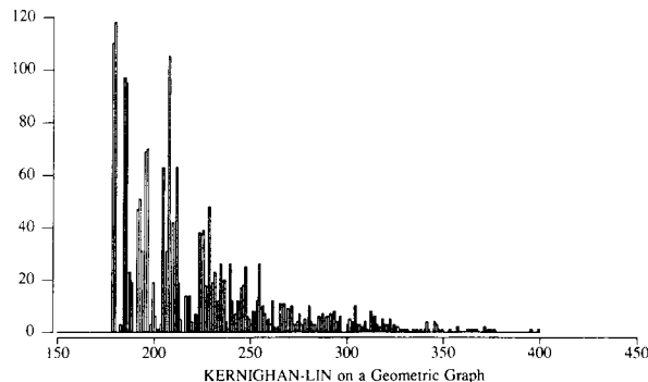
Figure 10. Histogram of solution values found for a geometric graph with n = 500 , n\pi d^2 = 20 during 2,000 runs of K-L. (The X-axis corresponds to cutsize and the Y-axis to the number of times each cutsize was encountered in the sample.)
