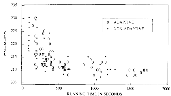
Figure 20. Results for adaptive and nonadaptive schedules as a function of running time.
