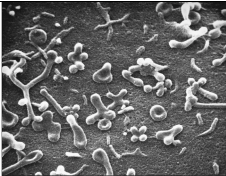
Figure 3.36 – Mycoplasma species lack cell walls
