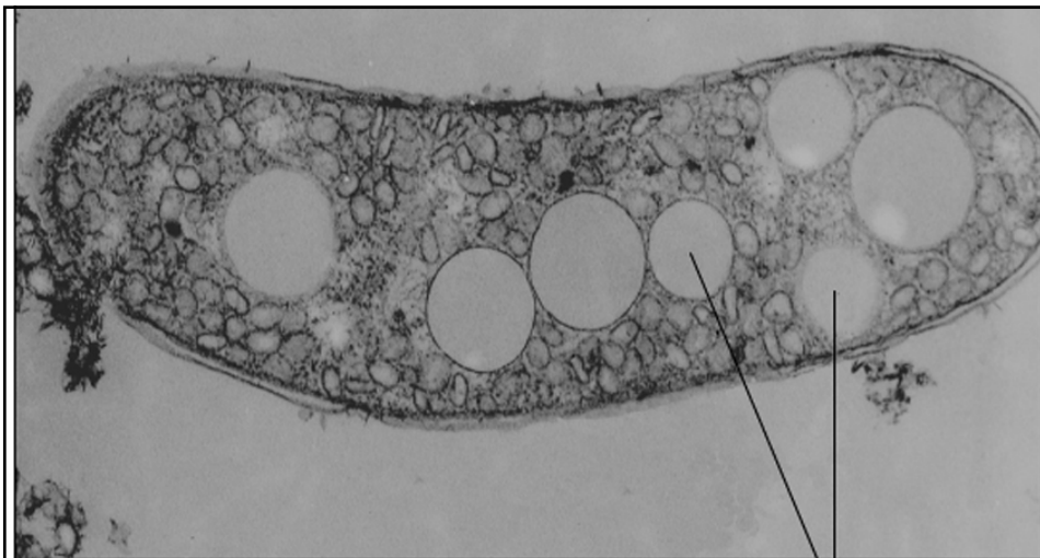
Figure 3.45 – Storage granules: Poly- \beta -hydroxybutyrate in Rhodospirillum rubrum
