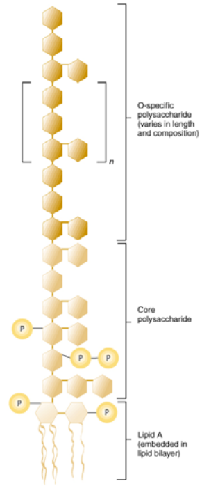
Figure 3.35 – Chemical structure of lipopolysaccharide (LPS)
