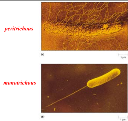
Figure 3.38 – Bacterial flagella
