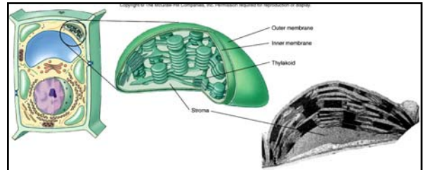
Figure 3.56 - Chloroplasts
