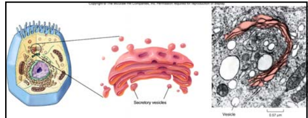
Figure 3.58 Golgi apparatus
