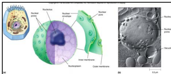
Figure 3.53 - Nucleus
