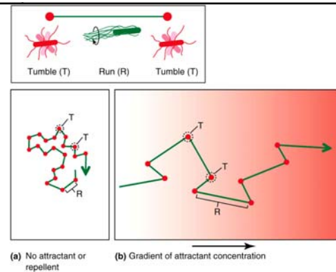
Figure 3.40 - Chemotaxis
