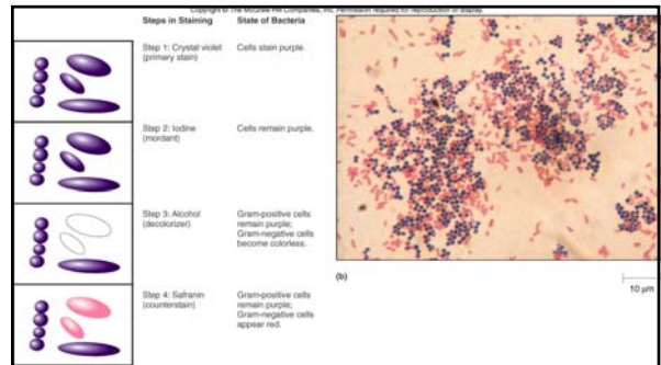
Figure 3.14 Gram stain
