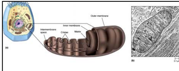
Figure 3.55 - Mitochondria
