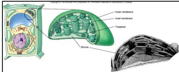
Figure 3.56 - Chloroplasts
